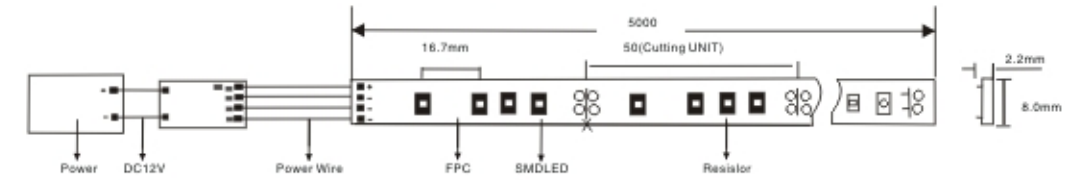
5050燈間距: 30燈33.3mm 48燈20.9mm 60燈16.7mm 5050 SMD Spacing: 30LED 33.3mm 48LED 20.9mm 60LED 16.7mm
